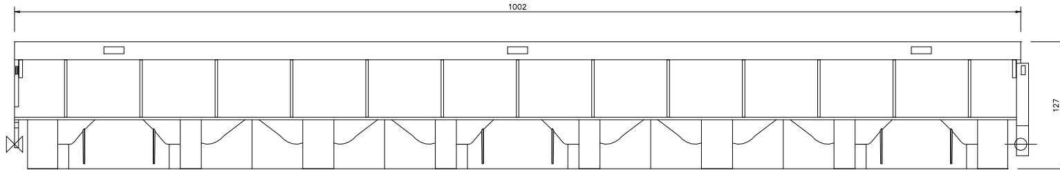
FLOPLAST LIMITED 110MM DOMESTIC CHANNEL DRAINAGE CHANNEL 1M LENGTH (INCLUDING GRATE) D700
