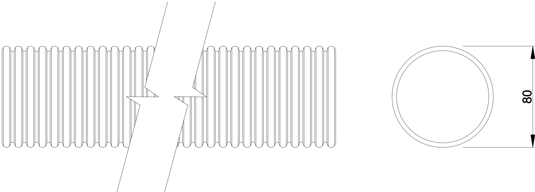
FLOPLAST LIMITED UNDERGROUND DRAINAGE SYSTEMS CORRUGATED COILED DRAINAGE PIPE PVC-U LAND DRAINAGE 80mm x 25m L8025
