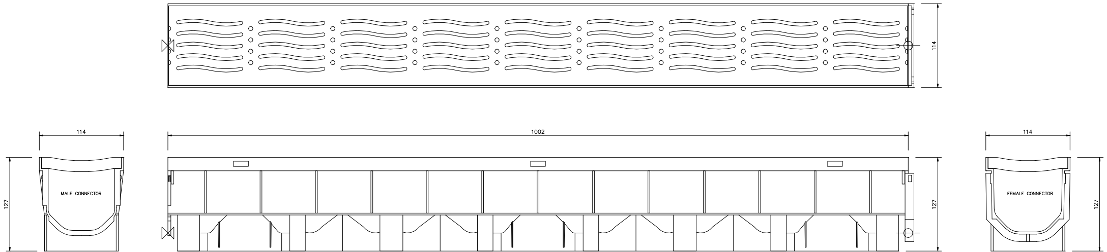
FLOPLAST LIMITED 110MM DOMESTIC CHANNEL DRAINAGE CHANNEL 1M LENGTH (INCLUDING GALVANISED GRATE) D701
