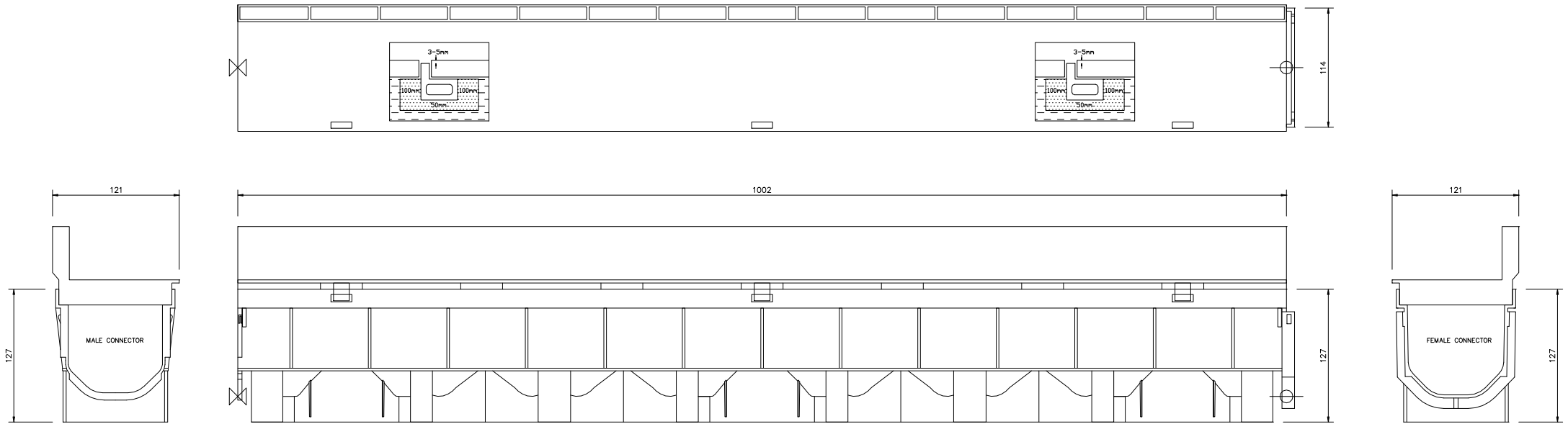
FLOPLAST LIMITED 110MM DOMESTIC CHANNEL DRAINAGE THRESHOLD CHANNEL DRAIN 1M LENGTH D730
