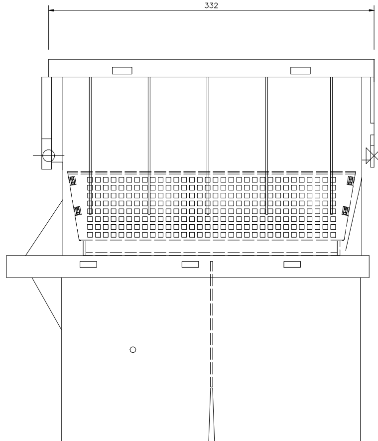
FLOPLAST LIMITED 110MM DOMESTIC CHANNEL DRAINAGE SUMP/TRAP UNIT AND BASKET WITH GALVANISED GRATE D733
