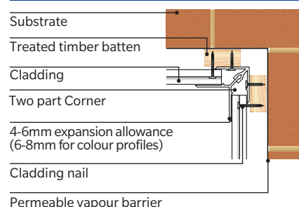
Top edge detail (B) Side Section
