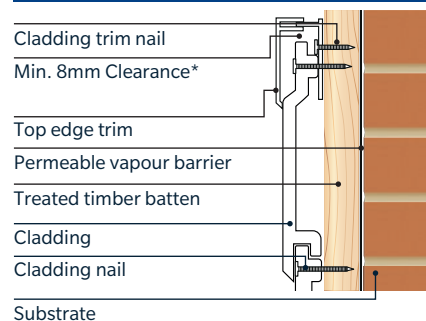
Top edge detail (B) Side Section
